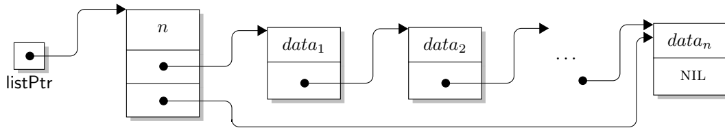
Figure 1.1: A singly-linked list model. In this model there is a header cell holding information about the list as a whole
