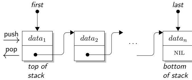
Figure 1.3: A stack model.
