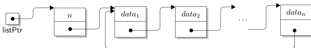
Figure 1.2: A circular singly-linked list model. In this model there is a header cell holding information about the list as a whole. Note that the last element is linked to the "first".
