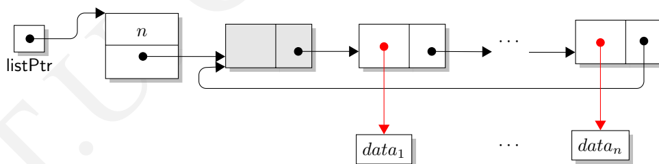
Figure 1.5: A model of a list for problem 1.3.
