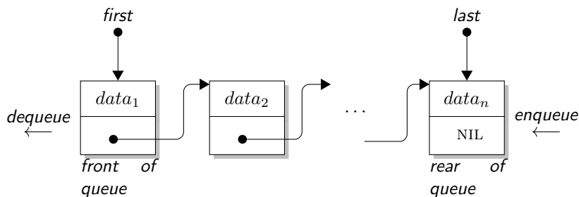
Figure 1.4: A queue model.
